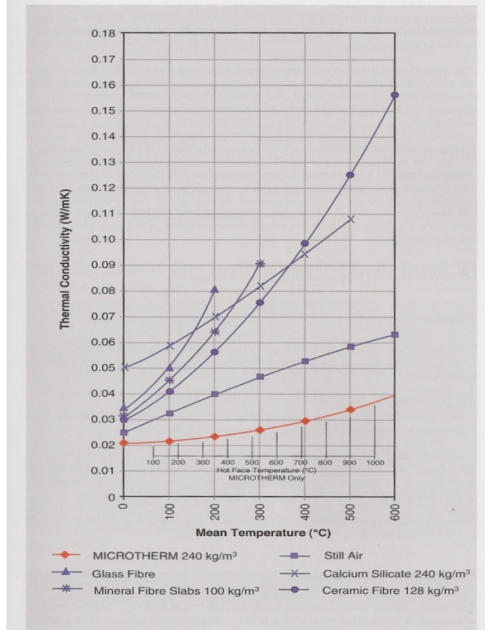
The Thermal Conductivity of MICROTHERM® Super G Insulation and Other Thermal Insulation Materials.
